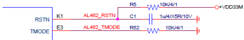
Figure 6. Reset Circuit for RSTN
